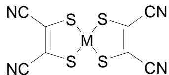
M(mnt) 2 (M=Fe, Ni, Cu)
