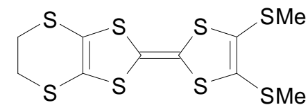
C1TET-TTF
