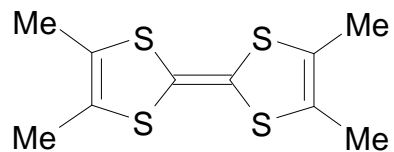
TMTTF
