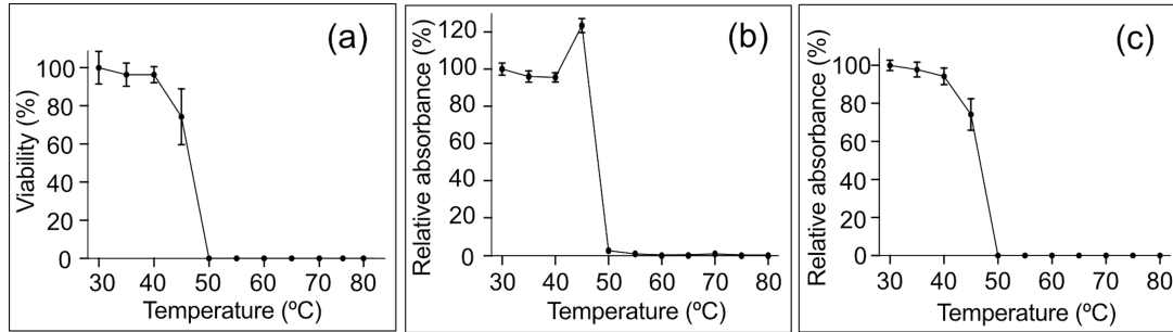
Figure 3. Viability analysis of A. platensis after heat-treatment.
